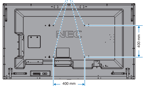
VESA-montage-interface (M8)
